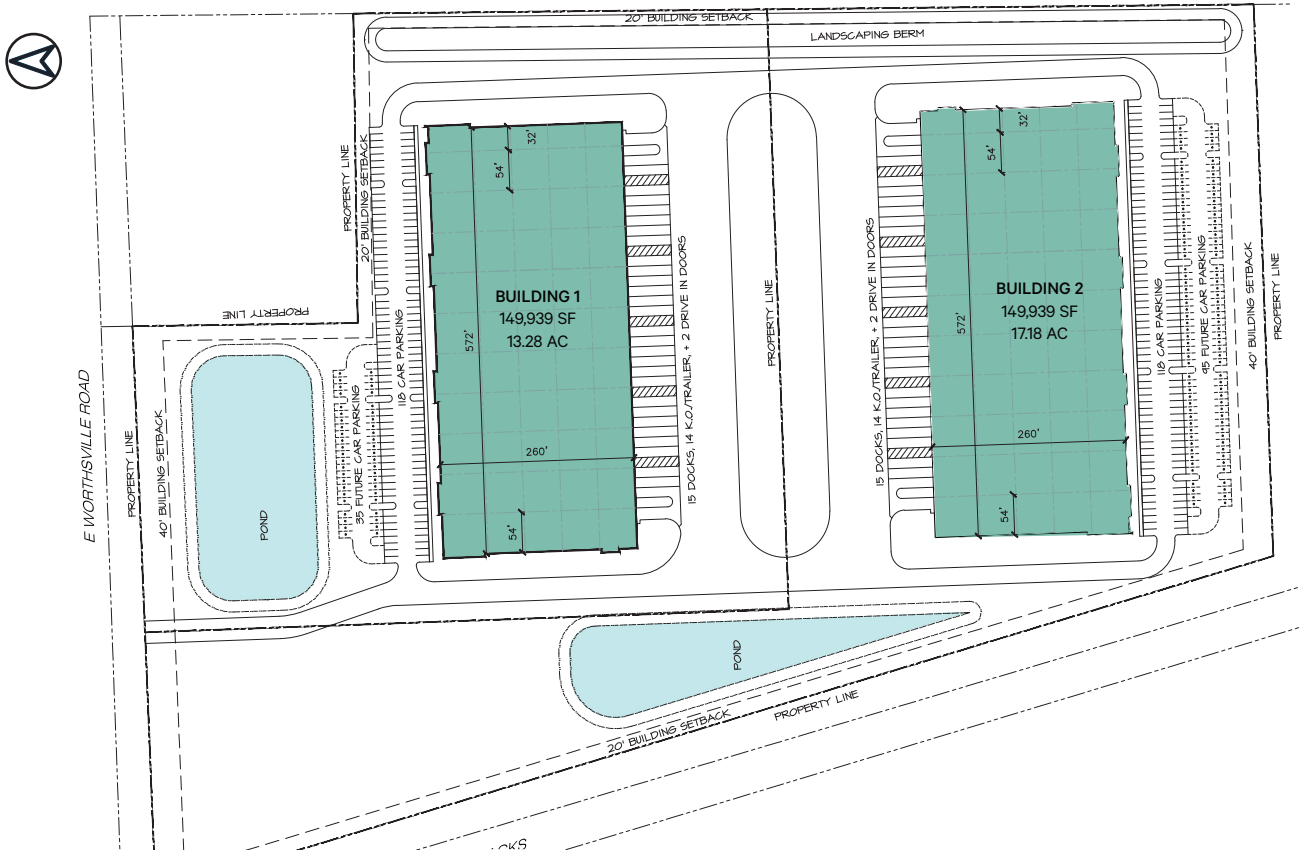
Sample Siteplan - 300,000 SF Rear-Load Configuration
